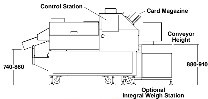
CT60 with integral weighing.
